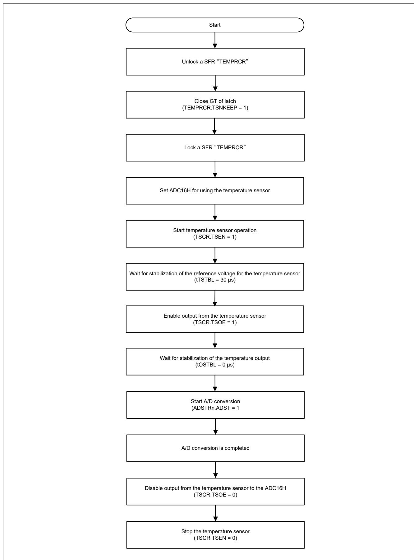
Figure 54.2 Procedure example for measuring temperature using TSN with ADC16H
