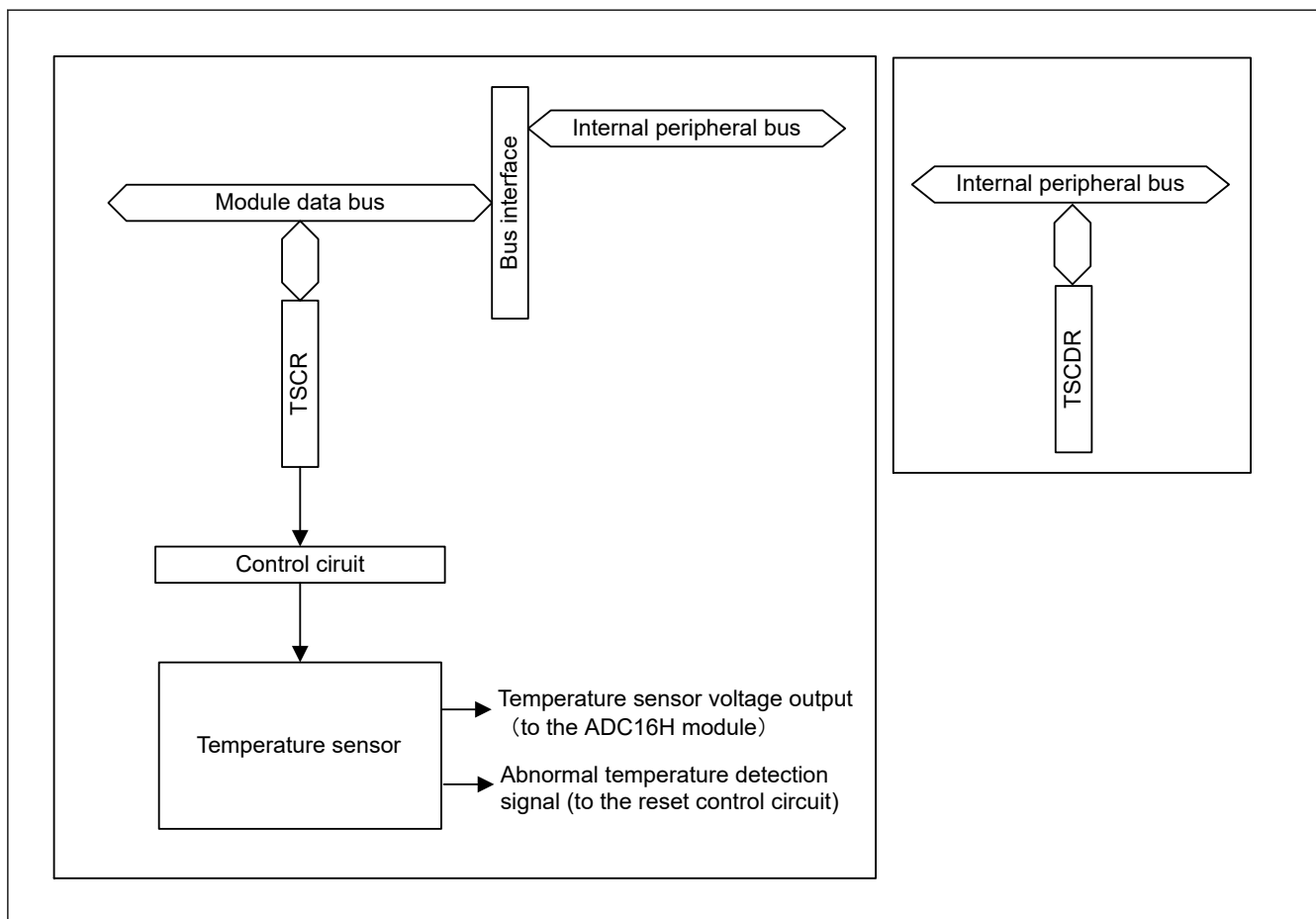
Figure 54.1 TSN block diagram
