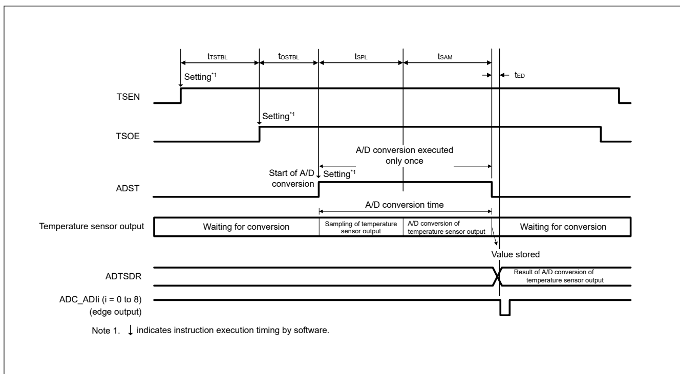
Figure 54.3 Timing from start of temperature sensor operation until completion of A/D conversion
