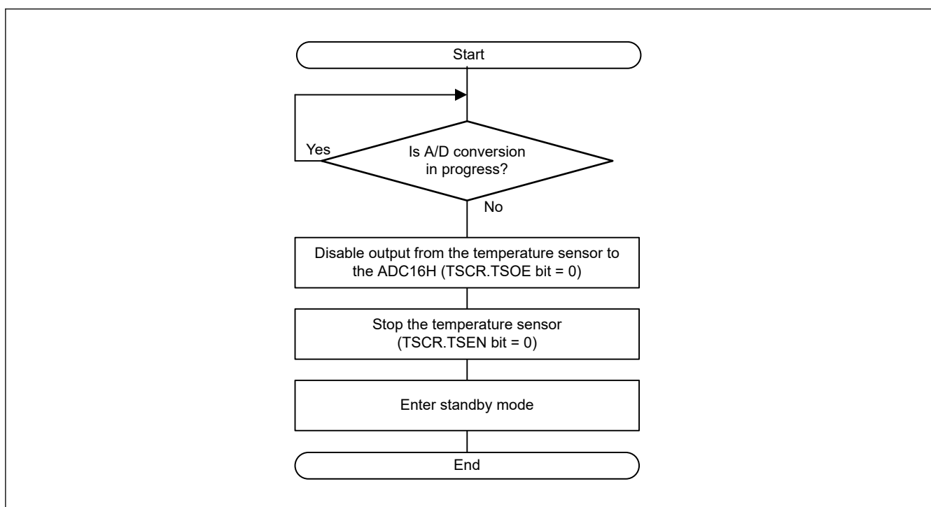
Figure 54.6 Example procedure for entering Software Standby mode
