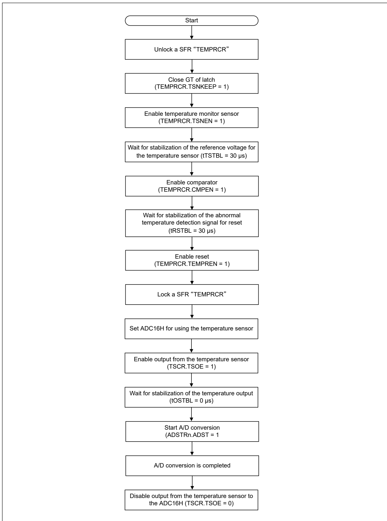
Figure 54.5 Procedure example for enabling temperature monitor reset and measuring temperature with ADC16H
