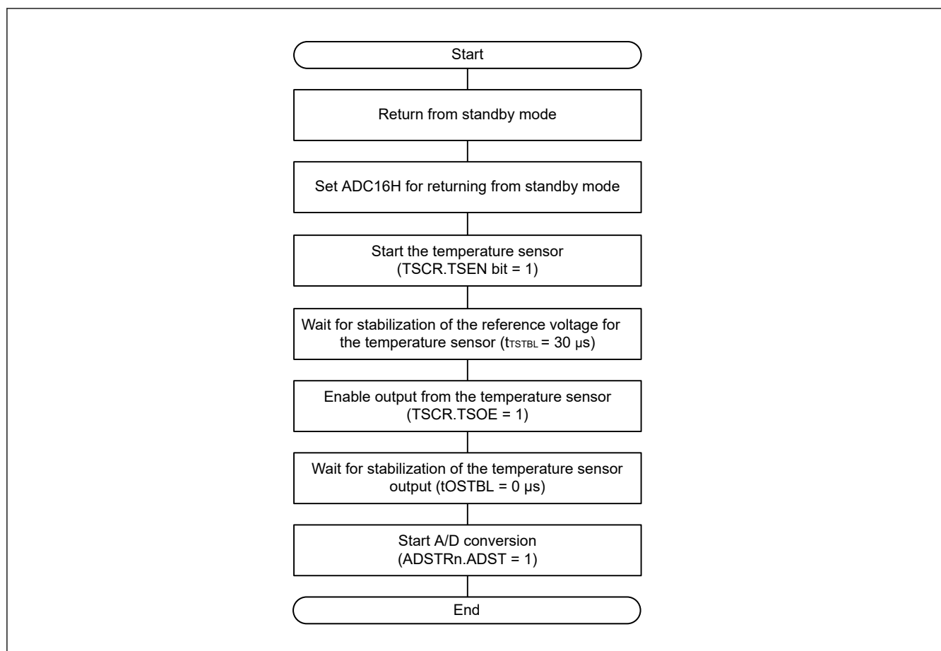
Figure 54.7 Example procedure for returning from Software Standby mode
