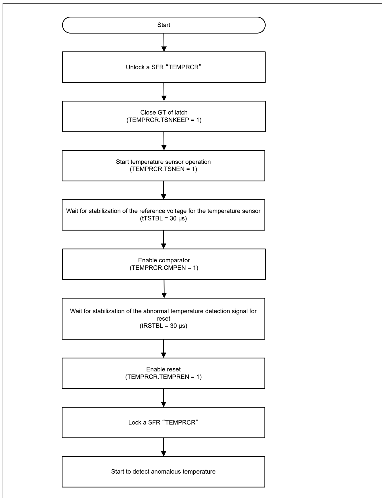
Figure 54.4 Procedure example for enabling temperature monitor reset but not measuring temperature with ADC16H
